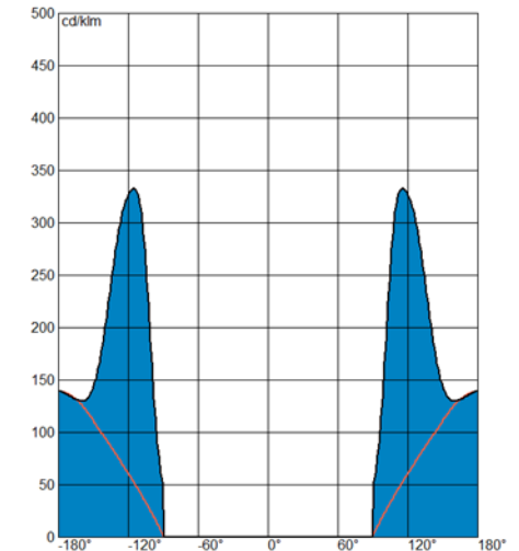
Intensity pattern LED: Nichia 757
