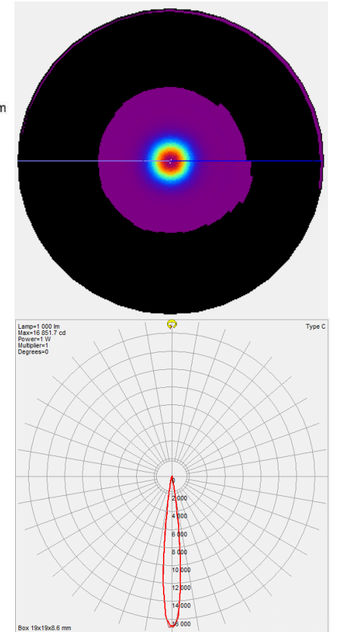
Intensity pattern
