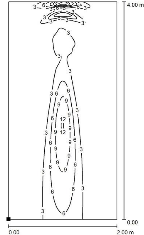
Dialux simulation
