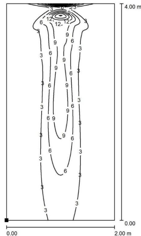
Dialux simulation
