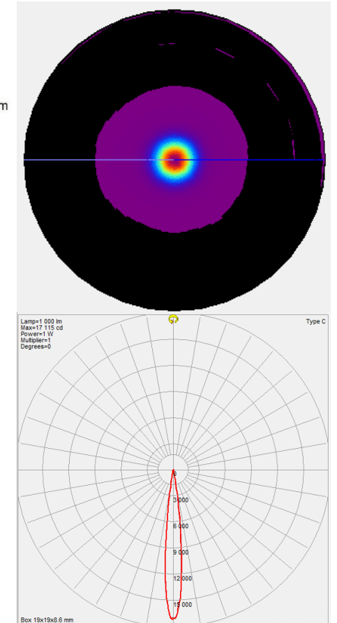
Intensity pattern
