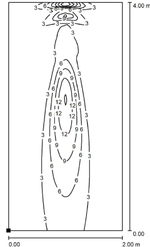
Dialux simulation
