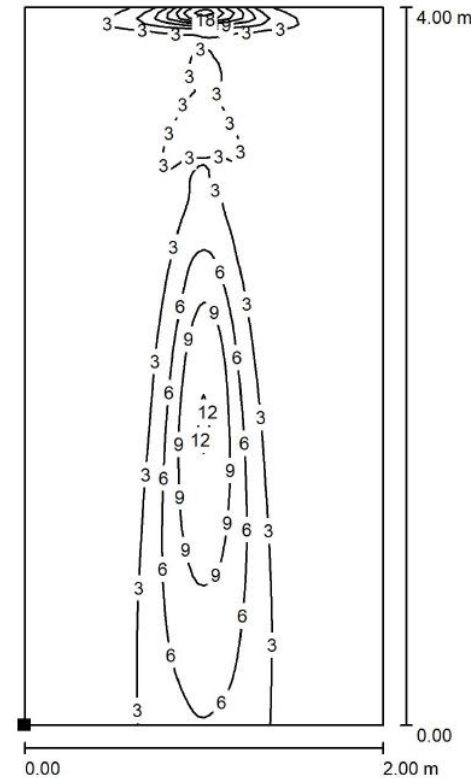
Dialux simulation
